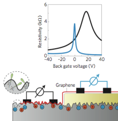
A single piece of gra- phene (red) is supported by SiO 2 substrate (left) and a flat BN multilayer (right). The corrugations, dangling bonds (inside dashed circle) and charge inhomogeneities that are inherent to SiO 2 surfaces shift and broaden the resistivity peak of the graphene (black line in plot) relative to that of graphene on BN (blue line)
